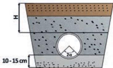
Trench dimensions
